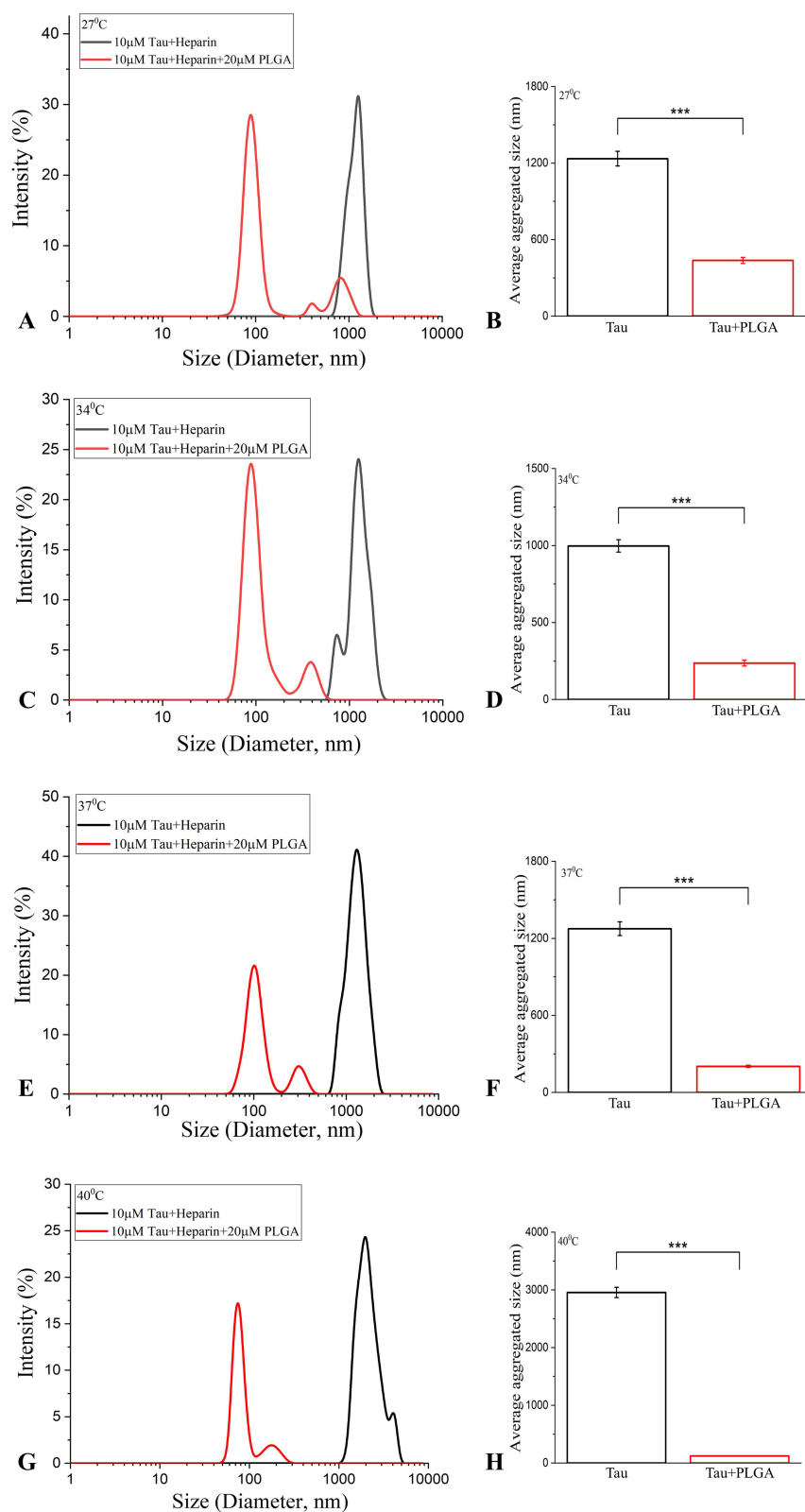
Figure 4 DLS analysis of tau aggregation in the presence of PLGA at different temperatures. (A–H) DLS analysis of 10μM 0N4R tau in the presence and absence of 20μM PLGA following 40hr incubation at 27°C (A and B) , 34°C (C and D) , 37°C (E and F) and 40°C (G and H) . Note the significant decrease in the diameter of tau aggregates in the presence of 20μM PLGA as a function of increase in temperature from 27°C to 40°C, compared to control tau as depicted by size distribution curves and respective histograms representing average sizes of tau aggregates for a given concentration. *** p < 0.001 .
