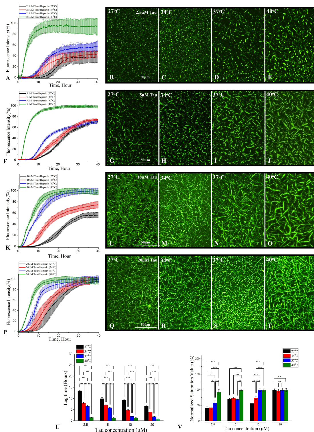
Figure 1 Aggregation of Tau in the presence of heparin at different temperatures. (A–T) ThT fluorescence kinetic assays showing the aggregation curves and the corresponding fluorescence images of 2.5 μM (A–E), 5 μM (F–J), 10 μM (K–O) and 20 μM (P–T) tau in the presence of heparin over a 40 hr incubation period at 27°C, 34°C, 37°C and 40°C. Note the aggregation of ON4R tau increases as functions of dose and temperature and plateaus over time as indicated by ThT fluorescence levels. The fluorescence images of tau fibrils at different concentrations were taken following 40 hr incubation at 27°C, 34°C, 37°C and 40°C. (U and V) Histograms showing the significant reduction of lag-time at various concentrations (2.5–10 μM) of tau with the rise of temperature from 27°C to 40°C (U) and the significant increase in final fluorescence values of various concentrations of tau with the rise of temperatures from 27°C to 40°C (V). All ThT kinetic graphs represented average mean ± SEM of three separate experiments, each performed with six replicates for each condition. n.s. represent non significant. *p < 0.05, **p < 0.01, ***p < 0.001.
