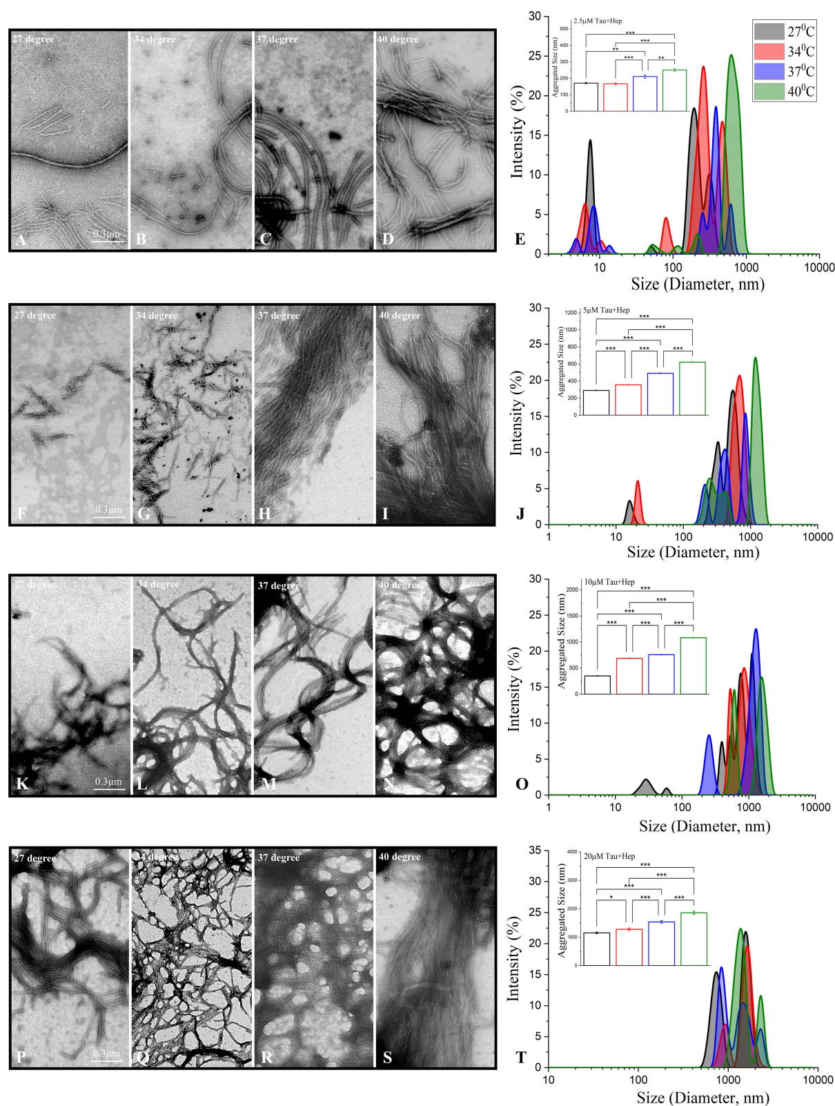
Figure 2 STEM and DLS analysis of tau aggregation at different temperatures. (A–T) STEM images and DLS analysis of 2.5 \mu\text{M} (A–E), 5 \mu\text{M} (F–J), 10 \mu\text{M} (K–O) and 20 \mu\text{M} (P–T) 0N4R tau in the presence of heparin over 40hr incubation at 27 ^{\circ}\text{C} , 34 ^{\circ}\text{C} , 37 ^{\circ}\text{C} and 40 ^{\circ}\text{C} . Note an increase in the aggregation, as revealed by STEM images, at each concentration of tau with the rise of temperature from 27 ^{\circ}\text{C} to 40 ^{\circ}\text{C} . DLS analysis showing variable significant increases in the diameter of aggregated tau at 2.5 \mu\text{M} (E), 5 \mu\text{M} (J), 10 \mu\text{M} (O) and 20 \mu\text{M} (T) with the rise of temperature from 27 ^{\circ}\text{C} to 40 ^{\circ}\text{C} following 40hr incubation as depicted by size distribution curves and histograms (insets) representing average aggregate sizes of tau aggregates for a given concentration. * p < 0.05 , ** p < 0.01 , *** p < 0.001 .
