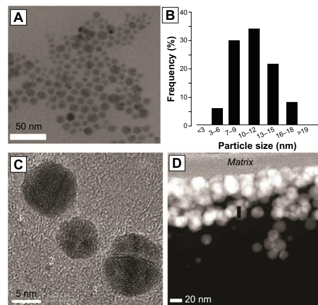
Figure 5 X-ray electron microscopy image of silver nanoparticles (A) and a particle size distribution histogram (B) of those particles. Higher magnification reveals polyhedral structure (C). Nondisruptive electron transmission microscopy reveals an 80–120 nm coating of silver nanoparticles on the surfaces of a polymer catheter (D).
