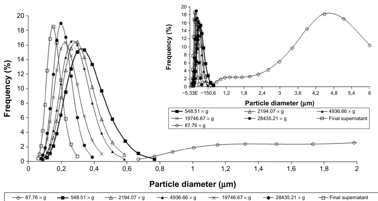
Figure 4 Study of particle separation by centrifugation of NP1.
