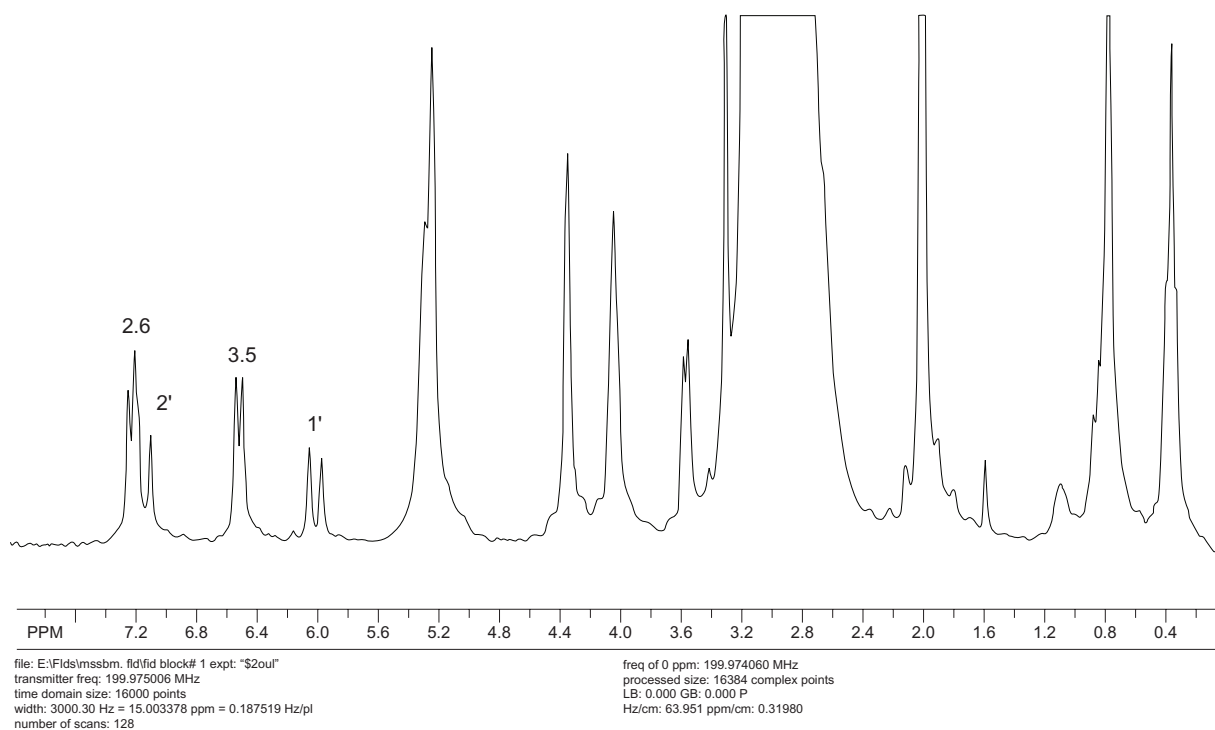
Figure 3 ^1\text{H} -NMR spectrum of the OMC ( A ), ^1\text{H} -NMR spectrum of the \beta -CD/OMC ( B ), molecular structure of the sunscreen ( C ) and complexation reaction ( D ). Abbreviations: OMC, octyl p-methoxycinnamate; \beta -CD, \beta -cyclodextrins.
