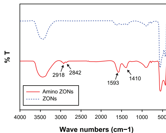
Figure 2 Fourier transform infrared spectra of nonmodified zinc oxide nanoparticles (dotted blue line) and amino-zinc oxide nanoparticles (solid red line).
