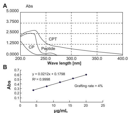
Figure 3 (A) Whole band ultraviolet scanning of chitosan-linked polyethylenimine, peptide, and chitosan/polyethylenimine/peptide complex. (B) The grafting rate of the chitosan/polyethylenimine/peptide complex.
