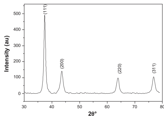
Figure 2 X-ray powder diffraction pattern by Cu K_{\alpha} radiation ( \lambda = 1.54060 Å) in 2\theta ranging from 30° to 80°.
