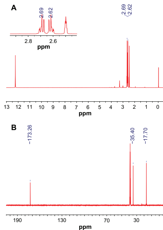
Figure S2 NMR spectrum of SeDPA. (A) ^1\text{H} NMR spectrum; (B) ^{13}\text{C} NMR spectrum. Abbreviation: SeDPA, 3, 3'-selenodipropionic acid; NMR, nuclear magnetic resonance.
