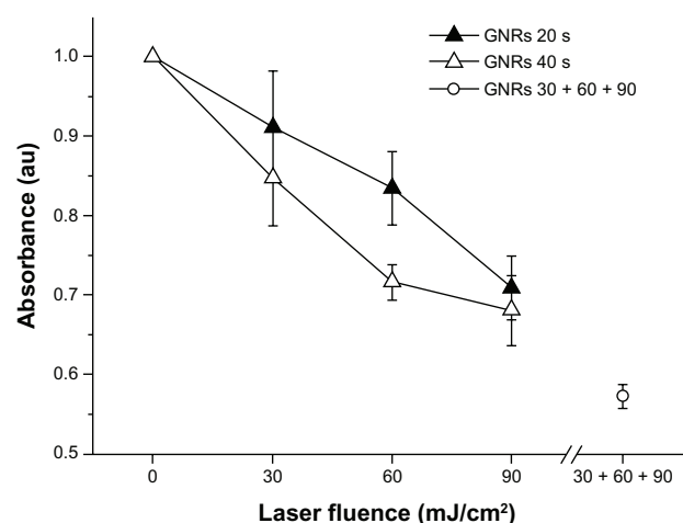
Figure 4 Normalized optical densities of gold nanorods (GNRs) at 1064 nm after exposure to laser fluences of 30, 60, and 90 mJ/cm² for 20 seconds (black triangles) and 40 seconds (white triangles), and consecutively to the three different laser fluences for 20 seconds each time (white circle).
