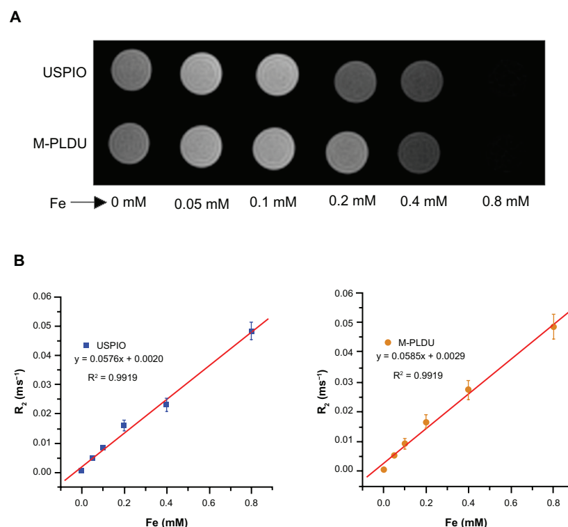
Figure 3 MRI properties of USPIOs and M-PLDUs in vitro: (A) signal intensity T_2 -weighted images (TR = 2500 ms; TE = 36 ms) of USPIOs and M-PLDUs in PBS at various iron concentrations at 25°C; blank PBS was taken as a control; (B) T_2 relaxation rate ( R_2 ) of USPIOs and M-PLDUs vs iron concentration.
