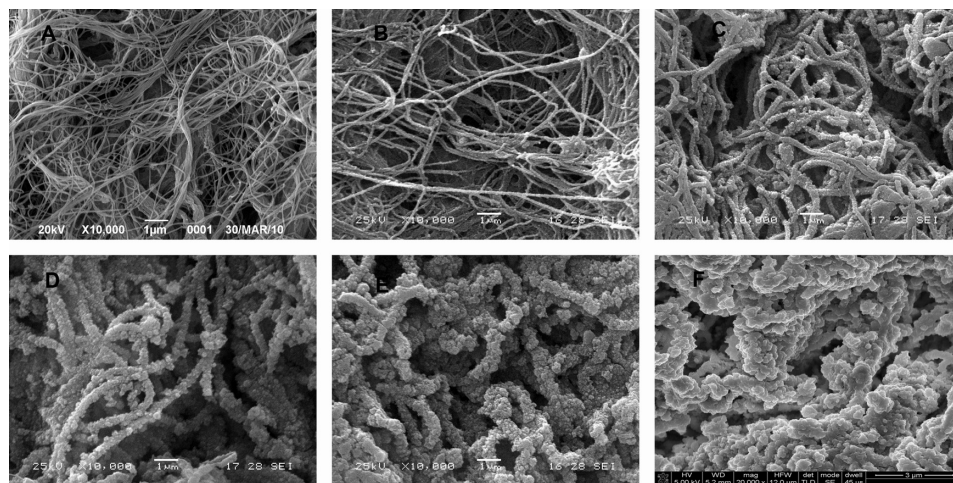
Figure 3 Luminal surface ultrastructure of scaffolds. (A) SEM image of unmodified scaffold (10,000 \times ). (B) SEM image of a scaffold modified by one cycle of heparin/DHI (10,000 \times ). (C) SEM image of scaffold modified by four cycles of heparin/DHI (10,000 \times ). (D) SEM image of scaffold modified by seven cycles of heparin/DHI (10,000 \times ). (E) SEM image of scaffold modified by ten cycles of heparin/DHI (10,000 \times ). (F) SEM image of scaffold modified by one cycle of heparin/DHI (20,000 \times ).
