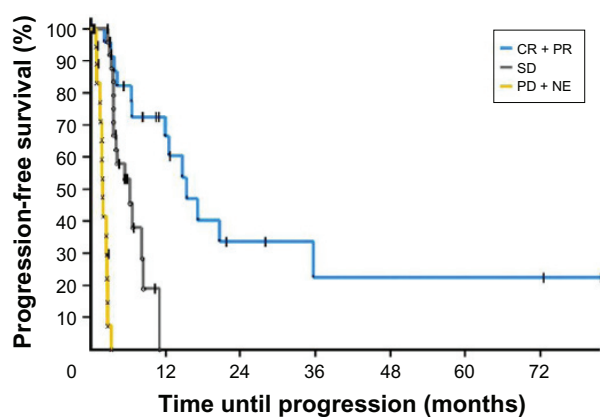
Figure 3 Kaplan-Meier curves from a phase II trial of romidepsin in patients with cutaneous T-cell lymphoma showing progression-free survival of patients with complete response (CR) or partial response (PR), patients with stable disease (SD), and patients with progressive disease (PD) or nonevaluable (NE) patients.
