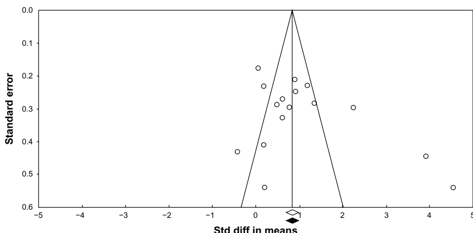
Figure 6 Funnel plot of standard error by standard difference in means.
