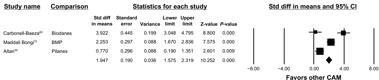
Figure 5 Other CAM forest plot.
