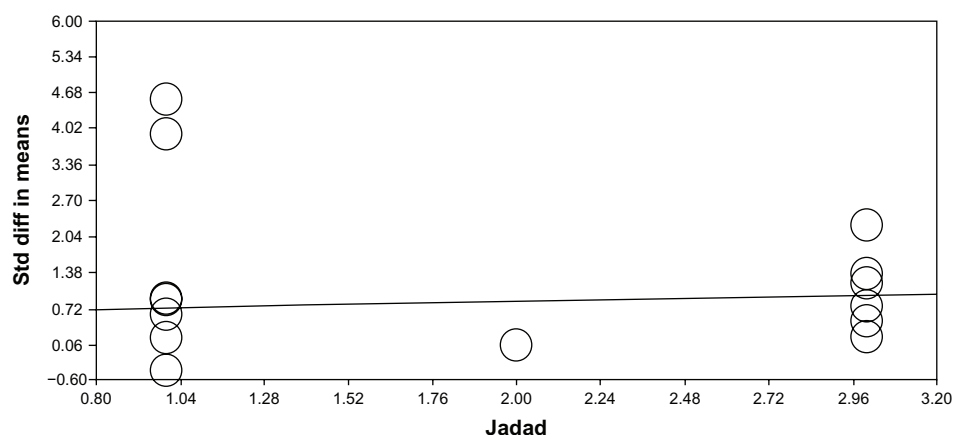
Figure 7 Regression of Jadad score on standard difference in means (Jadad et al, 1996). 57
