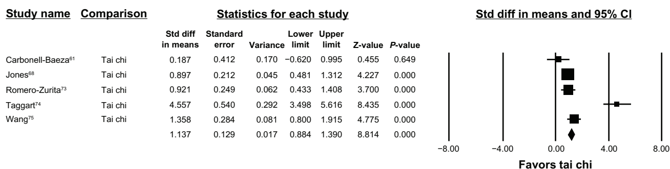
Figure 3 Tai chi forest plot.
