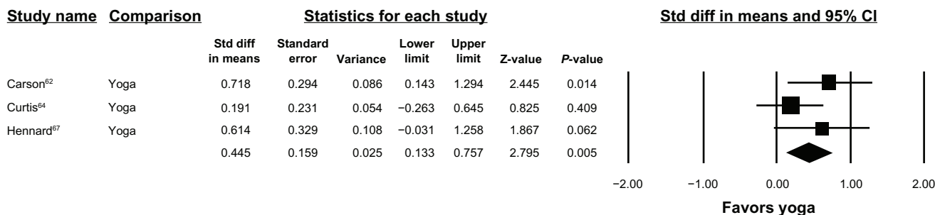
Figure 4 Yoga forest plot.
