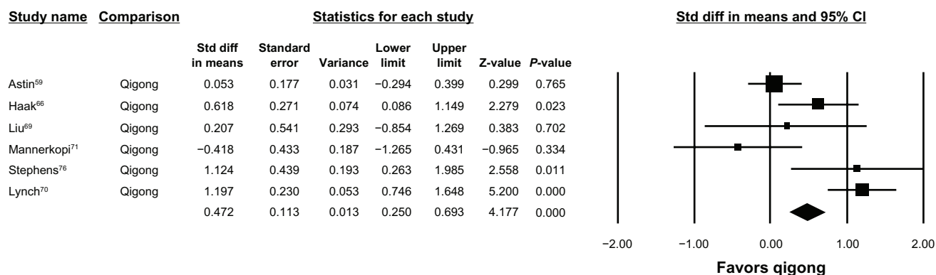
Figure 2 Qigong forest plot.
