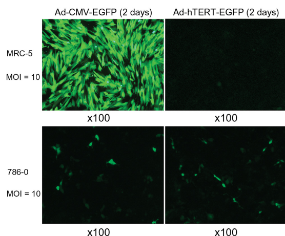
Figure 1 Expression of adenovirus cytomegalovirus-enhanced green fluorescent protein (Ad-CMV-EGFP) and Ad-human telomerase reverse transcriptase (hTERT)-EGFP in MRC-5 and 786-0 cells.
