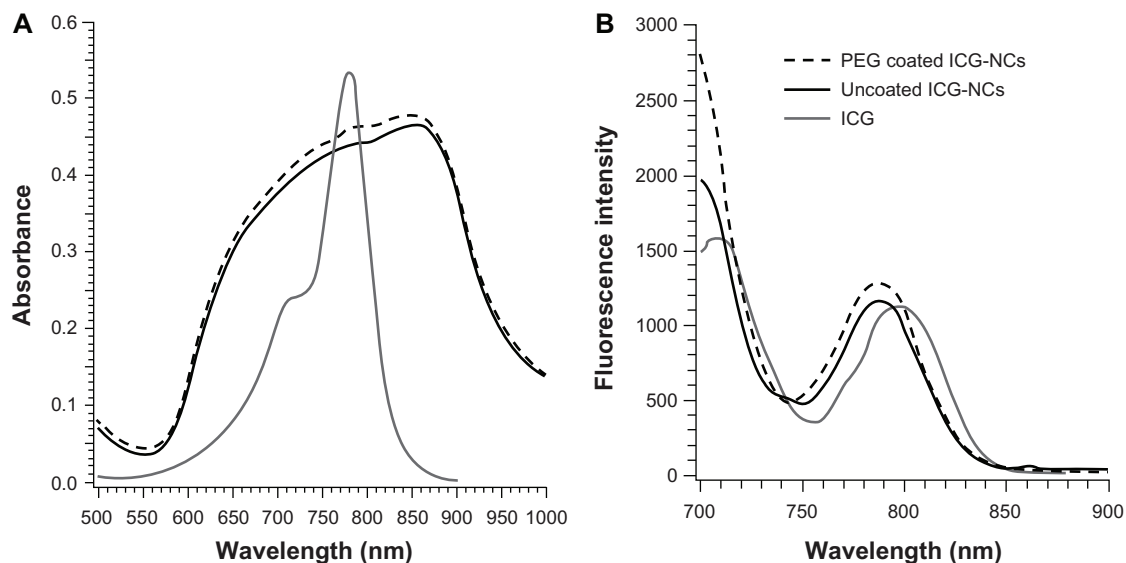
Figure 2 (A) Absorbance and (B) fluorescence spectra of indocyanine green (ICG) (9 \mu M), uncoated and polyethylene glycol (PEG)-coated indocyanine green-doped nanocapsules (ICG-NCs) ( \lambda_{\text{ex}} = 680 nm).
