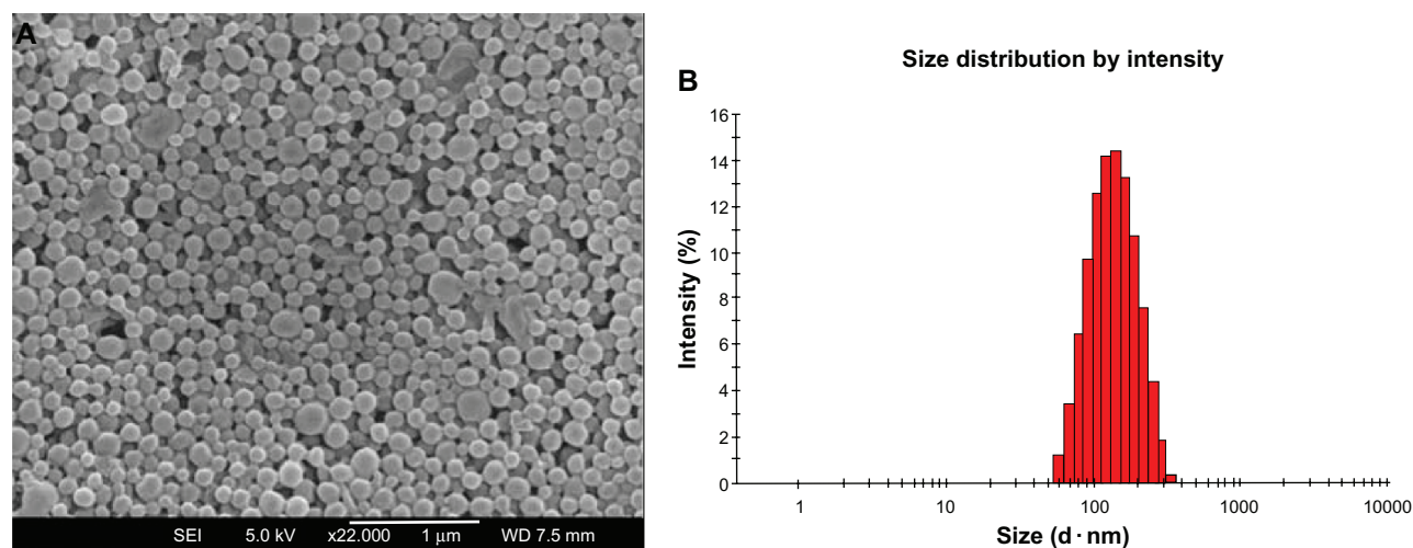
Figure 3 Field-emission scanning electron microscopy (A) and dynamic light-scattering spectra (B) of paclitaxel-loaded poly(glycolide-co-ε-caprolactone)-b-D-α-tocopheryl polyethylene glycol 2000 succinate nanoparticles.
