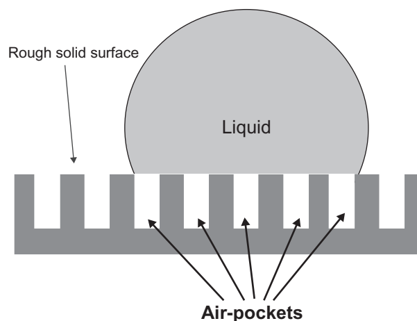
Figure 6 The Cassie–Baxter model of heterogeneous wetting. Notes: In this case, the liquid is considered to contact a surface consisting of the solid material and air. The width of spikes as well as the spacing between them is very small compared with the size of the liquid drop. To aid in visualization of the air pockets, the picture was not drawn to scale.
