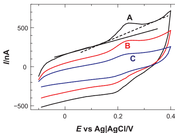
Figure 1 Cyclic voltammograms of saturated ferrocene in 0.1 M KCl at a platinum electrode 1.6 mm in diameter for scan rates, v = (A) 0.5, (B) 0.3, and (C) 0.1 V per second. Solid line and dashed line are backgrounds for evaluating oxidation peak current and charge, respectively.
