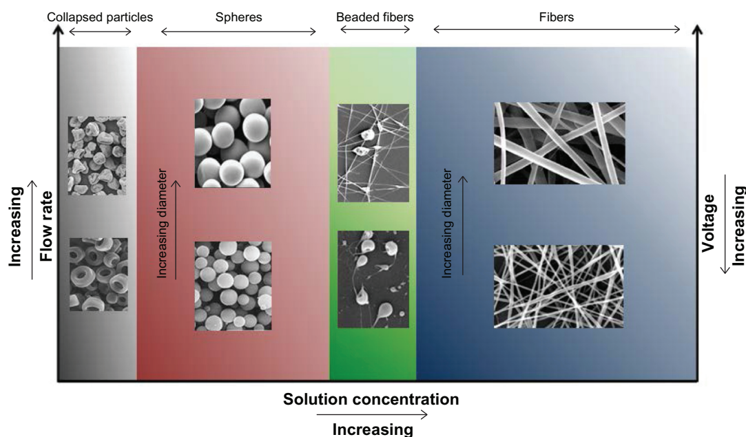
Figure 1 Schematic illustration of the effect of the concentration, flow rate, and voltage on electrosprayed/electrospun nano/microstructures.
