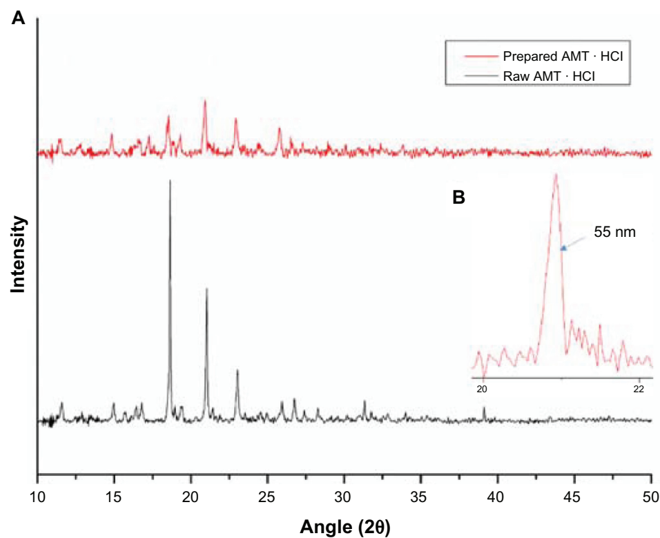
Figure 7 XRD of raw AMT · HCl and prepared AMT · HCl.
