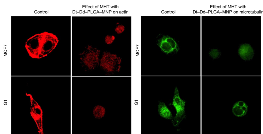
Figure 16 Confocal images of cytoskeletal staining with actin and microtubulin markers in control cells (before MHT) and cells after MHT with Dt–Dd–PLGA–MNP.
