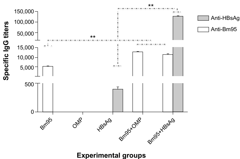
Figure 3 Immunostimulant properties of Bm95 in mice immunized by the intranasal route. The data are shown as the mean \pm standard deviation. **P < 0.01 , statistically significant difference by Student's t-test.
