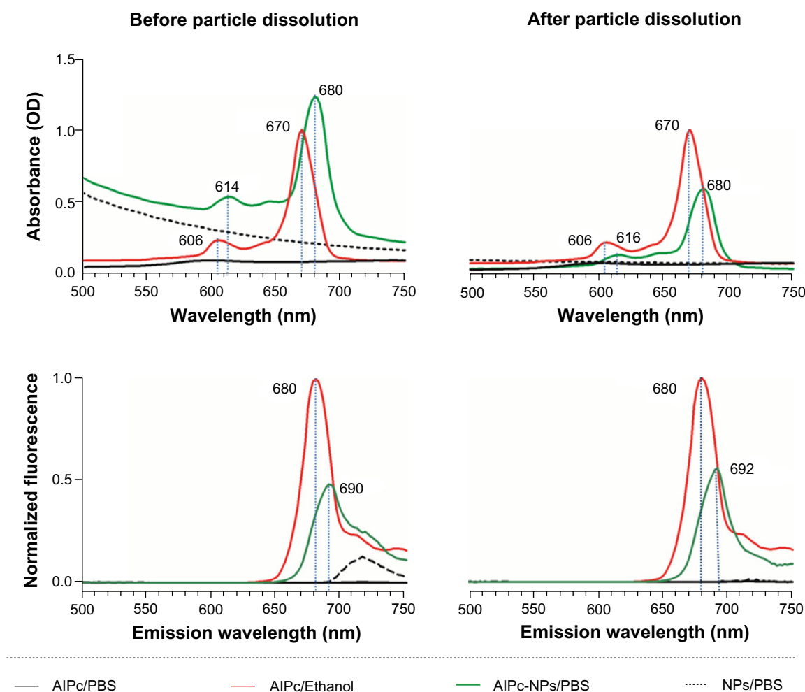
Figure 3 Absorbance and fluorescence (excitation at \lambda 350 nm) spectra of NPs and AlPc-NPs ( 1 \mu\text{M} AlPc) dispersed in PBS, before and after NP dissolution, and of 1 \mu\text{M} free AlPc in PBS or ethanol.
