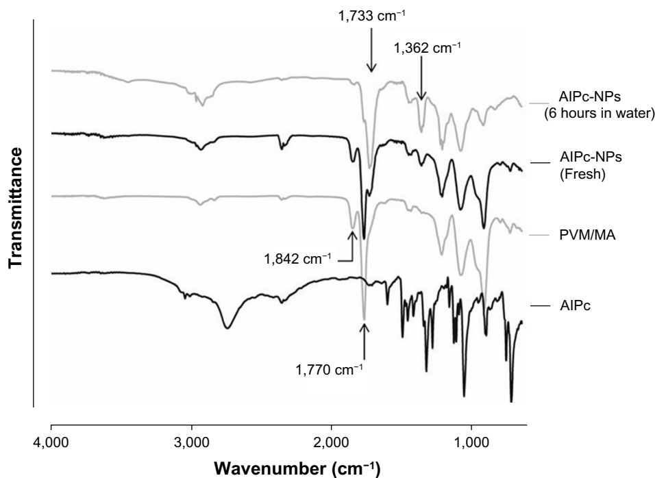
Figure 5 FTIR spectra of AlPc, PVM/MA, fresh AlPc-NPs, and AlPc-NPs exposed to water for 6 hours.
