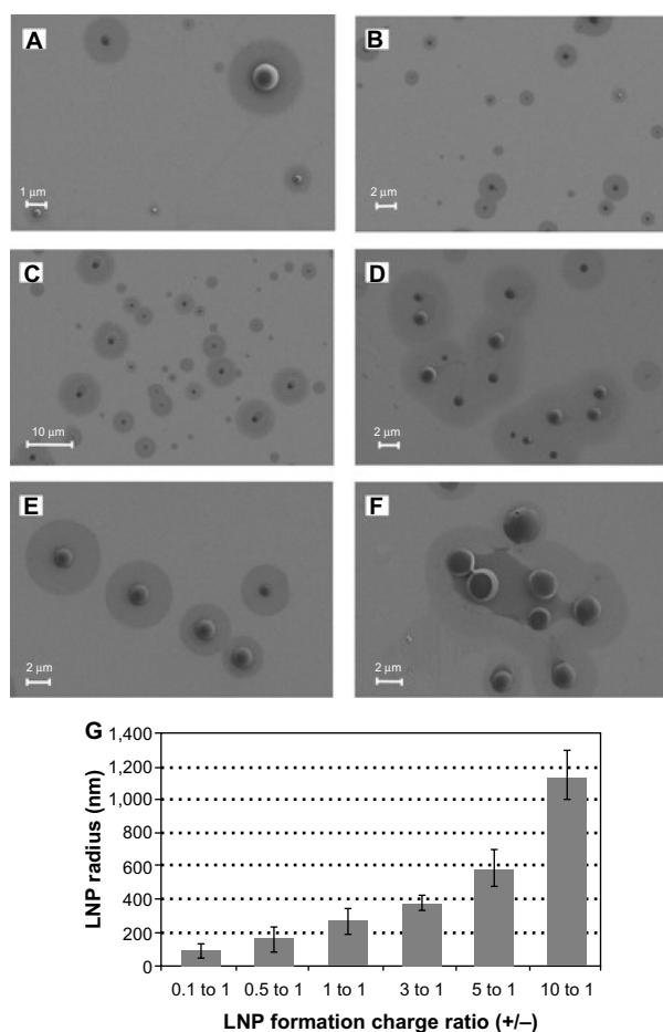
Figure 6 Lipitoid-siRNA complexes at varying charge ratios.
