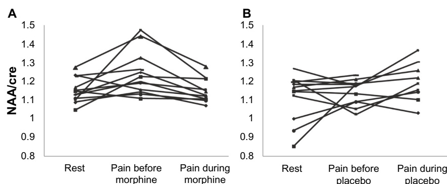
Figure 4 NAA/creatinine for each subject during rest and painful stimulation before and during treatment with morphine (A) and placebo (B). Abbreviations: cre, creatinine; NAA, N-acetylaspartate.
