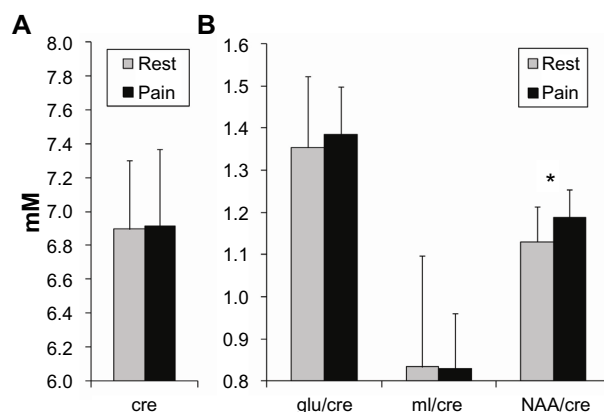
Figure 3 Creatine concentration (A) and metabolite ratios (ratio, no unit) (B) at rest (gray) and during painful stimulus before treatment (black). * P<0.05 . Abbreviations: ml, myo-inositol; cre, creatine; glu, glutamine; NAA, N-acetylaspartate.
