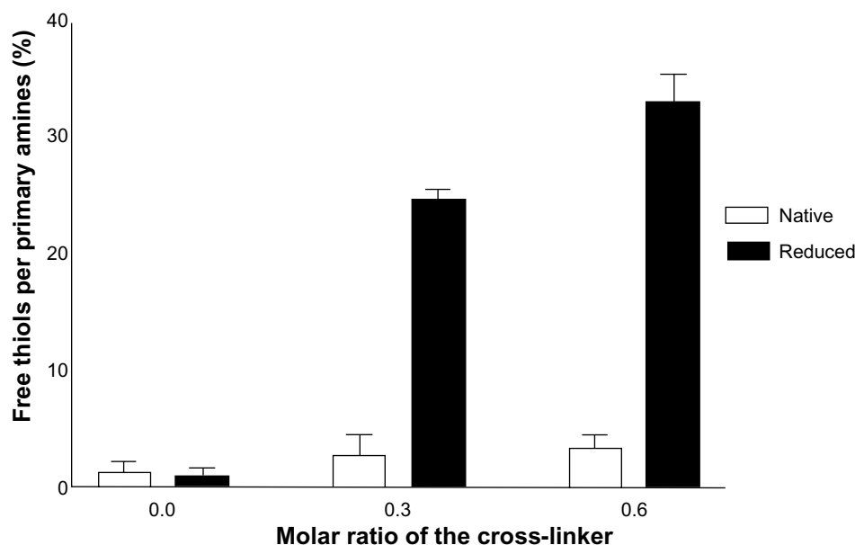
Figure 7 Redox-sensitive degradation of the nano-networks demonstrated by Ellman's assay of free thiols prior to and after addition of 0.2 M \text{NaBH}_4 .
