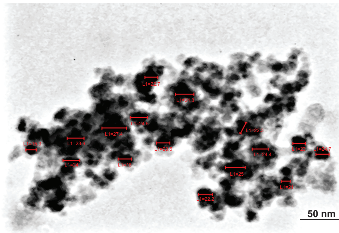
Figure S3 Scaling of transmission electron microscopy image of MScI for nanoparticle size–distribution histogram. Abbreviation: L, length.
