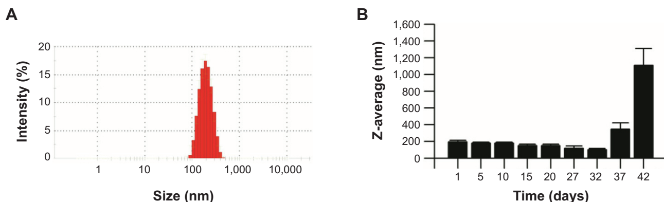
Figure 4 Size distribution (A) and stability of BAY-CS-SeNPs (B).
