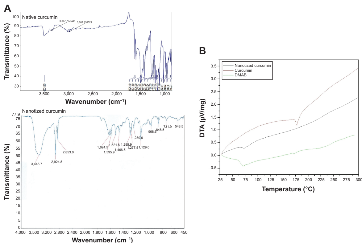
Figure 2 (A) FT-IR spectrum of native and nanotized curcumin. (B) DTA thermogram of native curcumin, nanotized curcumin, and DMAB. Abbreviations: DMAB, didodecyldimethylammonium bromide; DTA, differential thermal analysis; FT-IR, Fourier transform infrared.
