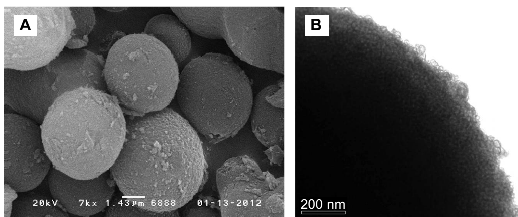
Figure 2 Electron microscopy images of spherical mesoporous silica beads on (A) field emission scanning electron microscopy and (B) transmission electron microscopy.
