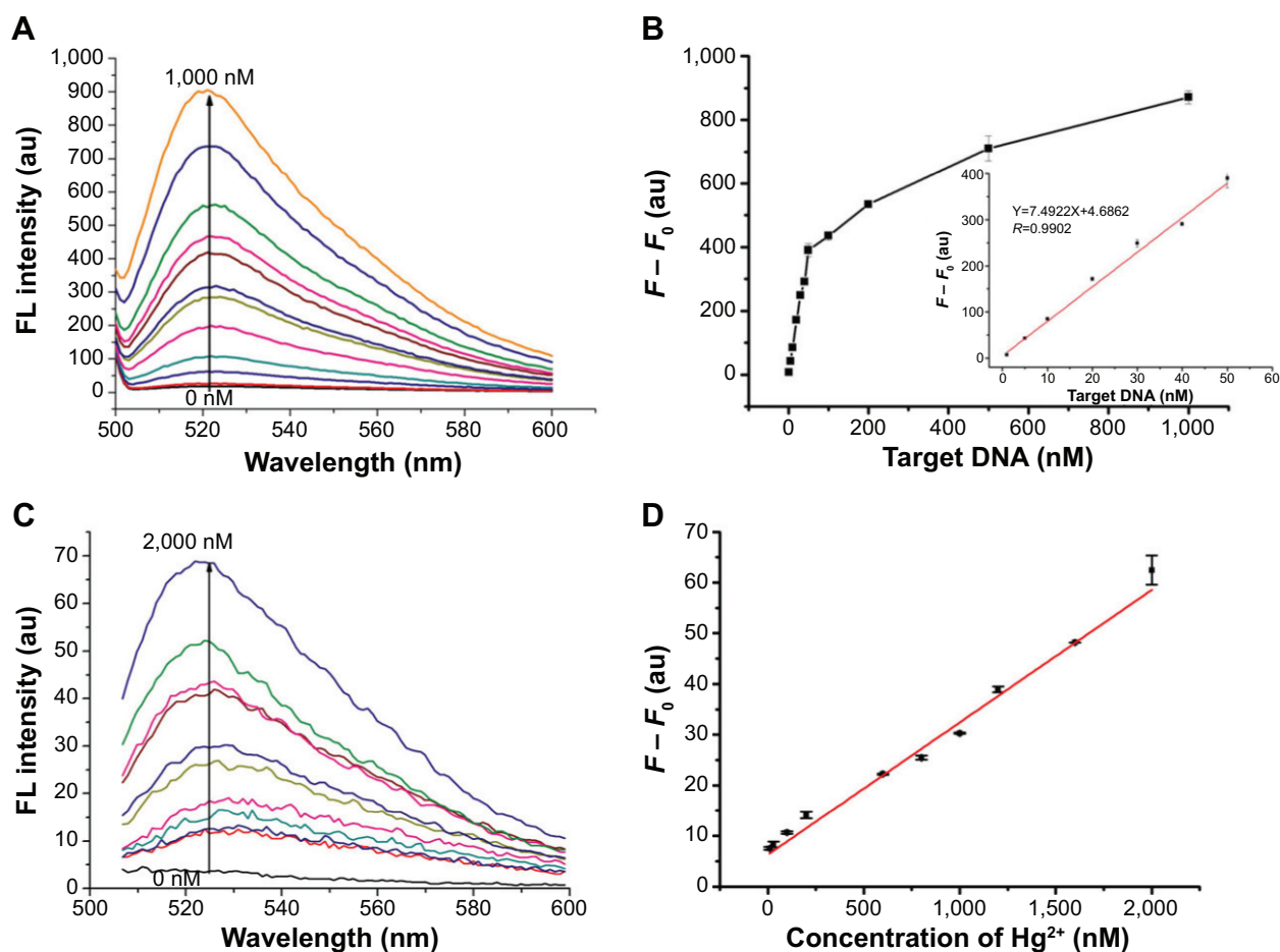
Figure 6 Fluorescence spectra (A, C) and the changeable fluorescence intensities (B, D) towards different concentrations of MDRI gene (A, B) and \text{Hg}^{2+} (C, D).
