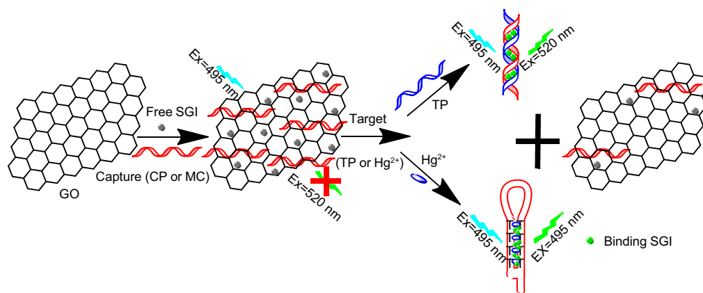
Figure 1 Representation of the signal-on fluorescence sensing strategy for MDR1 gene and \text{Hg}^{2+} based on SGI dye and GO.
