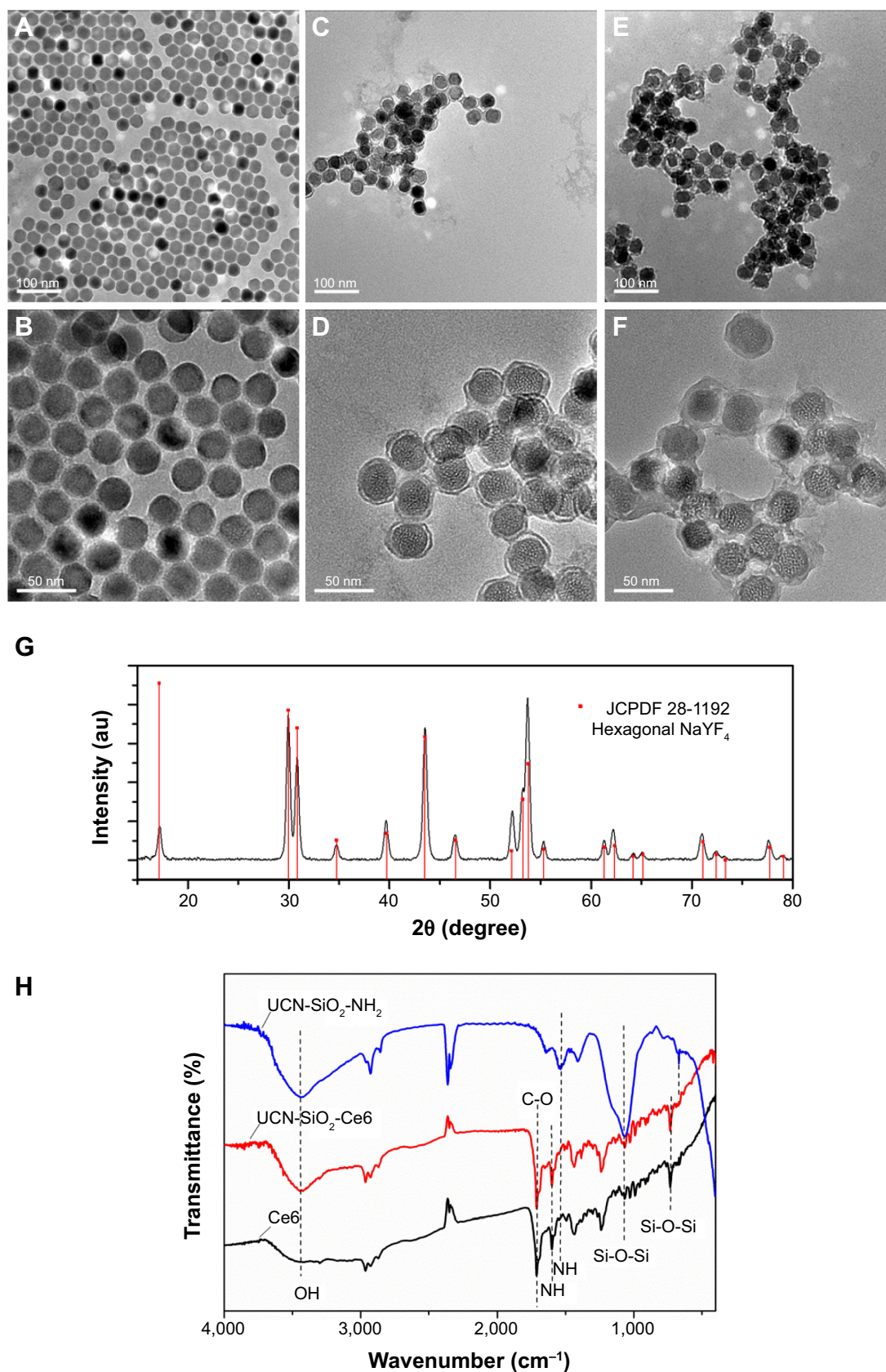
Figure 2 (A–F) Transmission electron microscope images of NaYF 4 :Yb,Tm UCN, amino group–modified silica–coated UCN and Ce6–conjugated UCN. (G) X–ray diffraction pattern of NaYF 4 :Yb,Tm UCN. (H) FTIR for UCN–SiO 2 –NH 2 , Ce6, and UCN–SiO 2 –Ce6.
