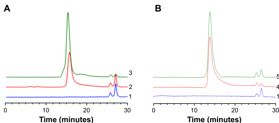
Figure 1 Representative chromatograms.
