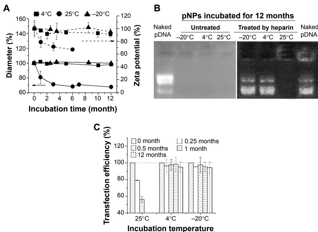
Figure 5 Storage stability of plasmid deoxyribonucleic acid (pDNA)-loaded lipopolymerosomes (pNPs).
