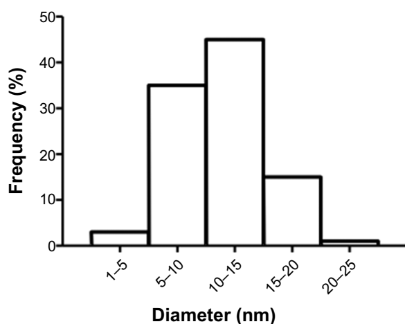
Figure 1 Histogram of titanium oxide-nanoparticle (TiO 2 NP) size distribution. The predominant size for TiO 2 NPs ranged from 10 to 15 nm. The size distribution was obtained from six independent dynamic light scattering measurements.
