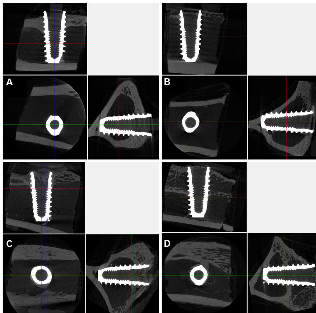
Figure 7 Micro-computed tomographic images 8 weeks after implant installation. (A) Machined surface group, (B) SLA surface group, (C) \text{TiO}_2 nanotube array surface group, and (D) \text{TiO}_2 nanotube array surface with rhBMP-2 group.
