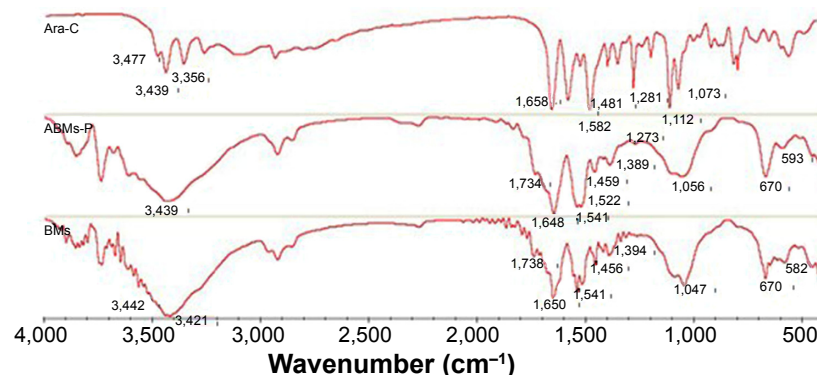
Figure 4 The FTIR spectrum of Ara-C, ABMs-P, and BMs.
