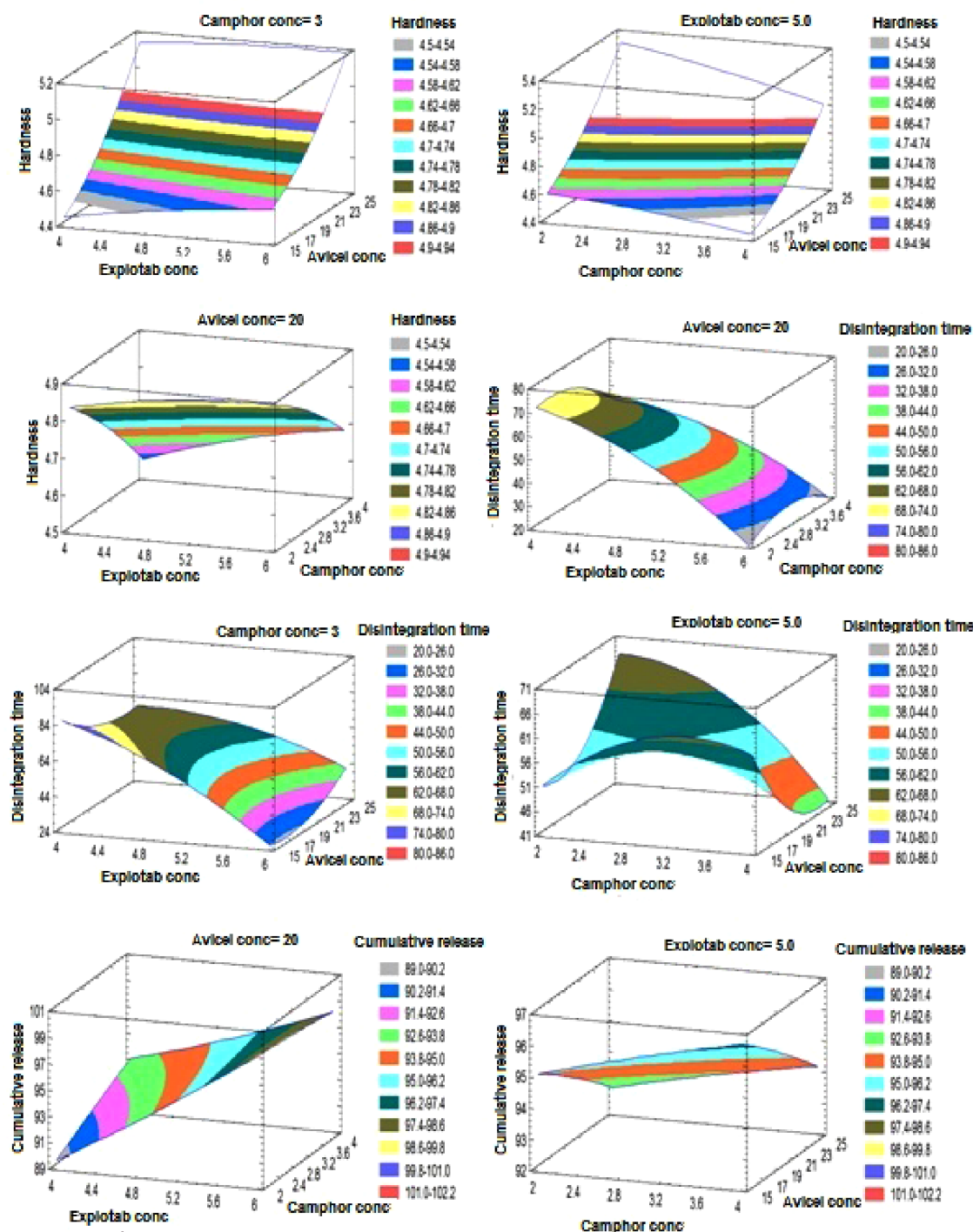
Figure 6 Estimated response surfaces with contour plots showing the effects of X_1 , X_2 , and X_3 on the dependent variables ( Y_1 – Y_3 )
