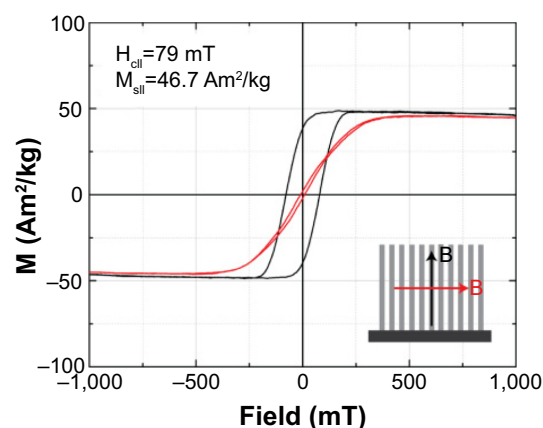
Figure 2 Magnetization loops of an array of Ni NWs embedded in the alumina membrane with magnetic field applied in the in-plane and out-of-plane directions.
