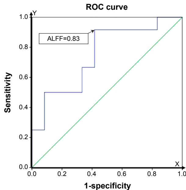
Figure 5 ROC curve of the mean ALFF value of the left IPL area.
