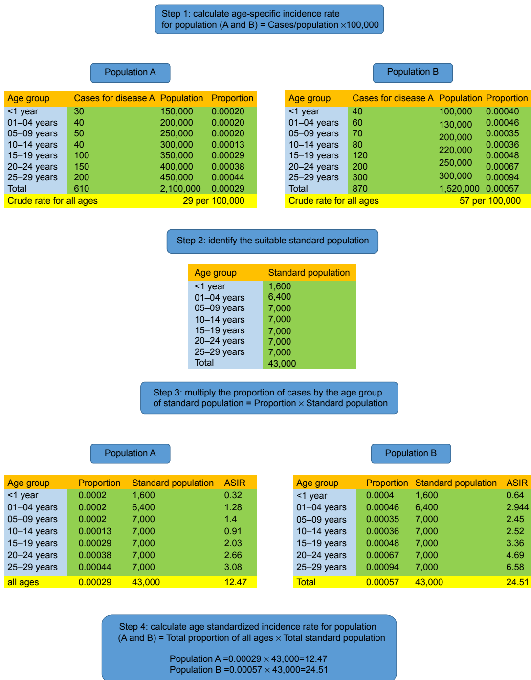
Figure 1 An example of direct age adjustment for calculating age standardized incidence rate. Abbreviation: ASIR, age standardized incidence rate.
