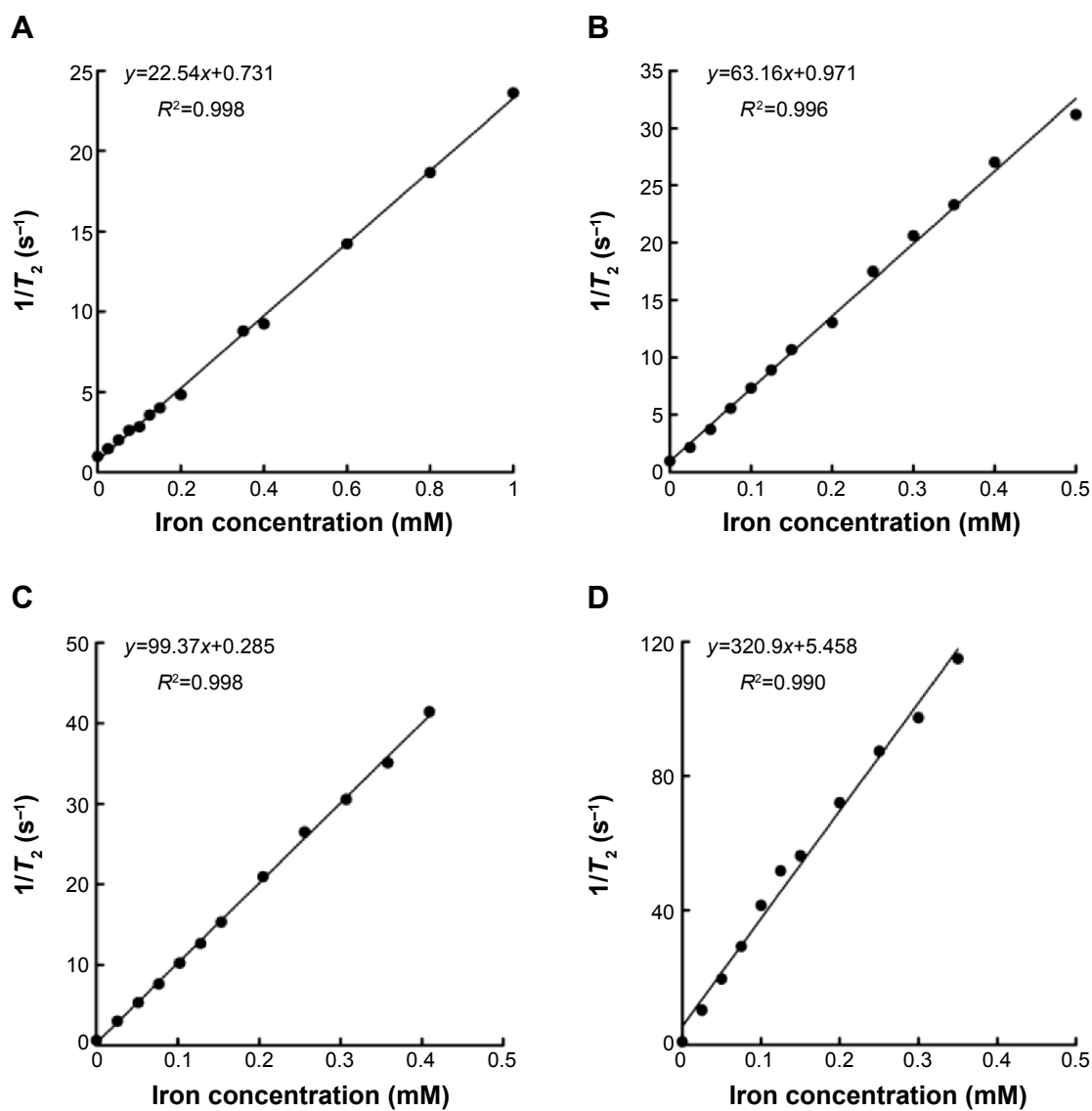
Figure S3 Analysis of transverse relaxivity of M-HFn nanoparticles by linear mapping iron concentration and 1/T_2 .
