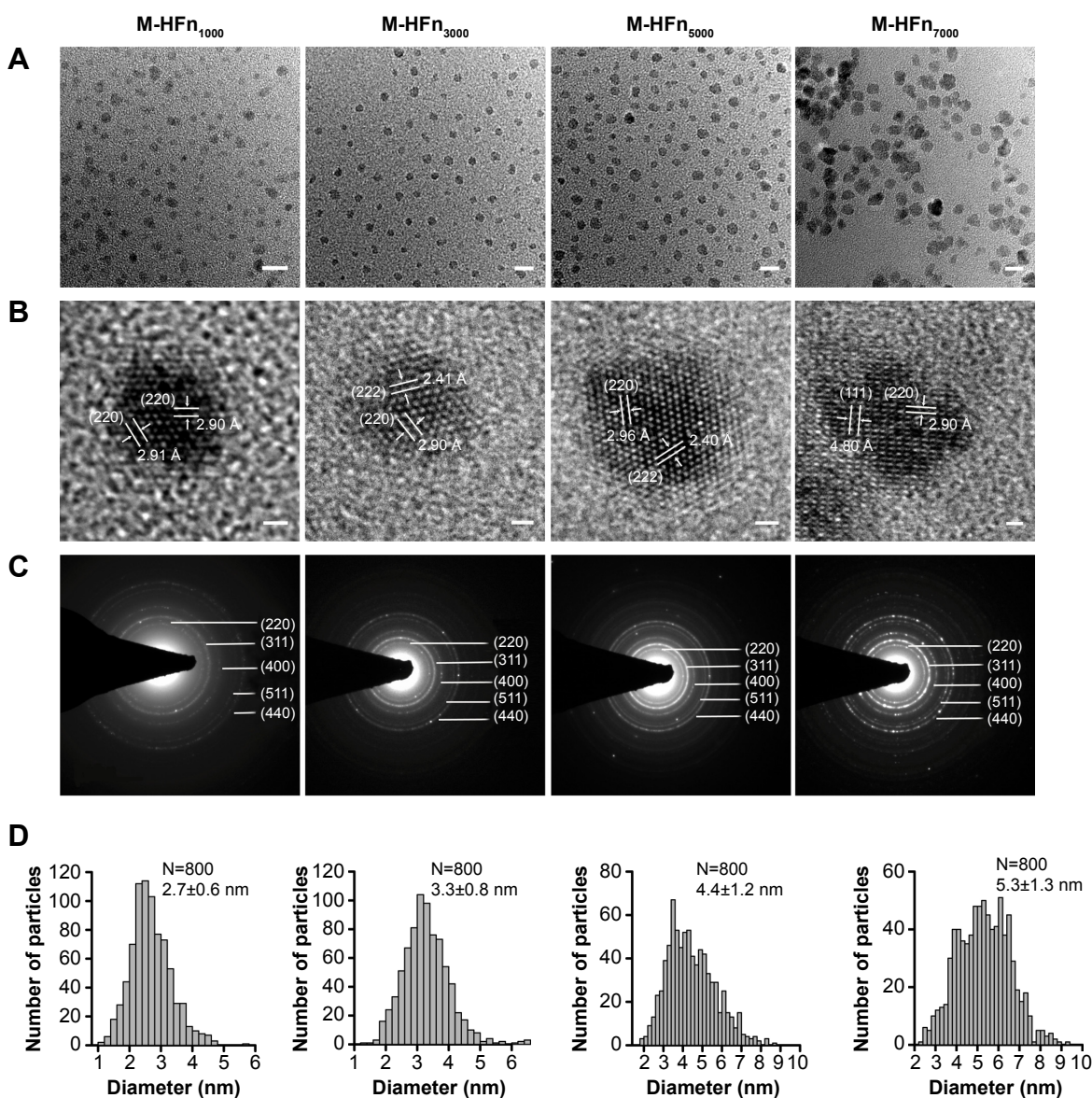
Figure 1 TEM analysis of M-HFn nanoparticles.
