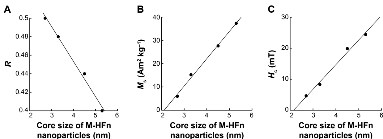
Figure 3 Size dependence of magnetic properties of M-HFn nanoparticles.
