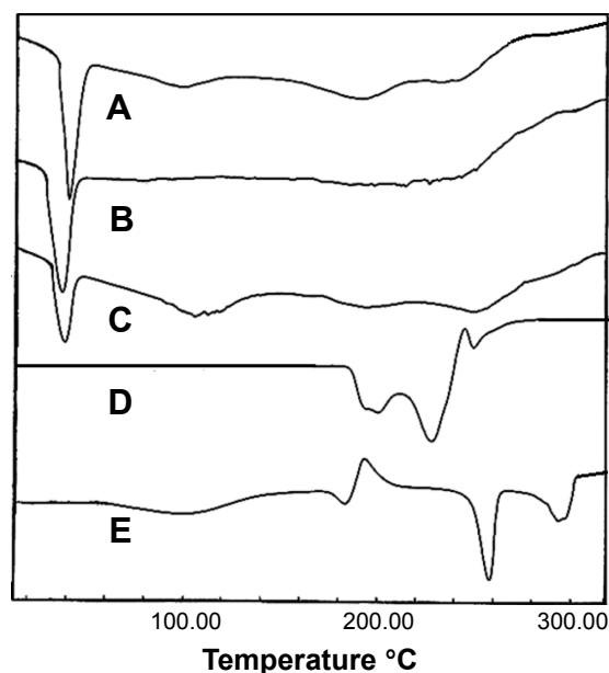
Figure 3 DSC curves.
