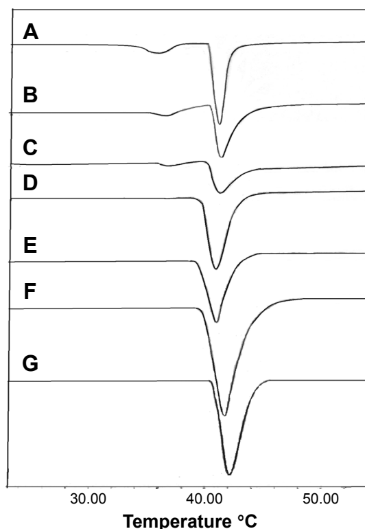
Figure 2 DSC curves.
