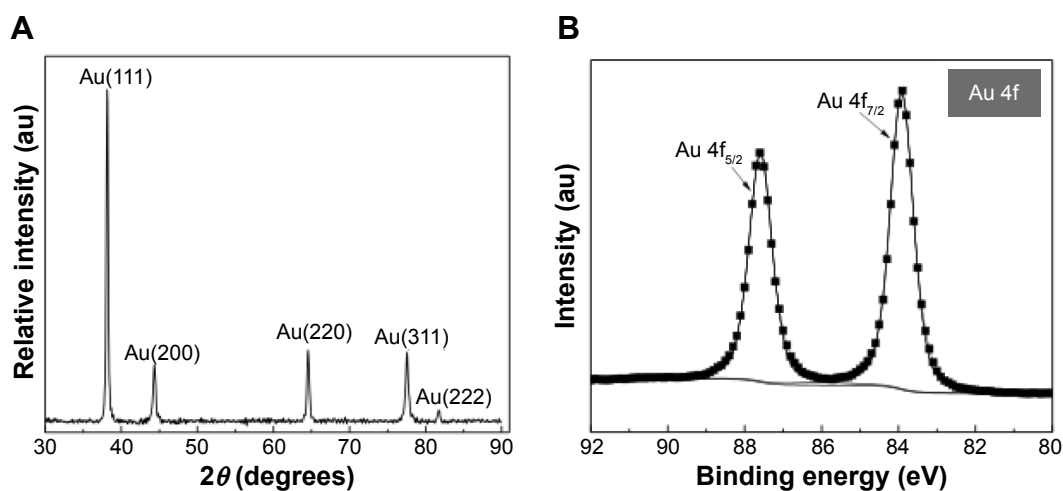
Figure 4 Surface analyses of Au deposited by PLD onto WOx.
