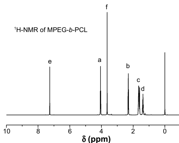
Figure 2 Typical 1 H-NMR spectra of block copolymer MPEG-b-PCL.
