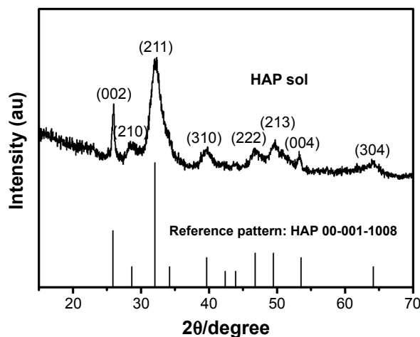
Figure 2 XRD pattern of HAP particles in sol.
