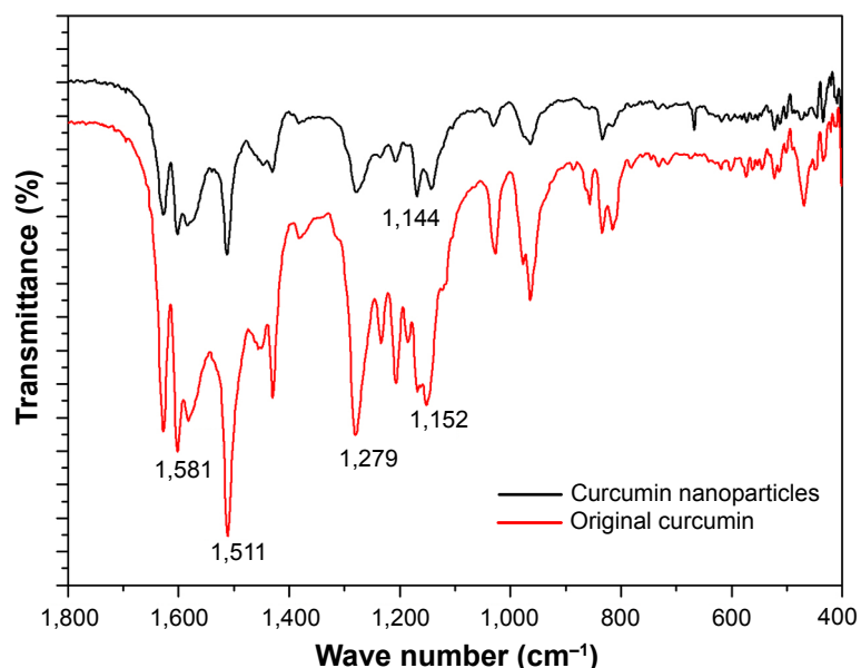
Figure 6 FTIR spectra of original curcumin and curcumin nanoparticles prepared by the SEDS process under optimal conditions.
