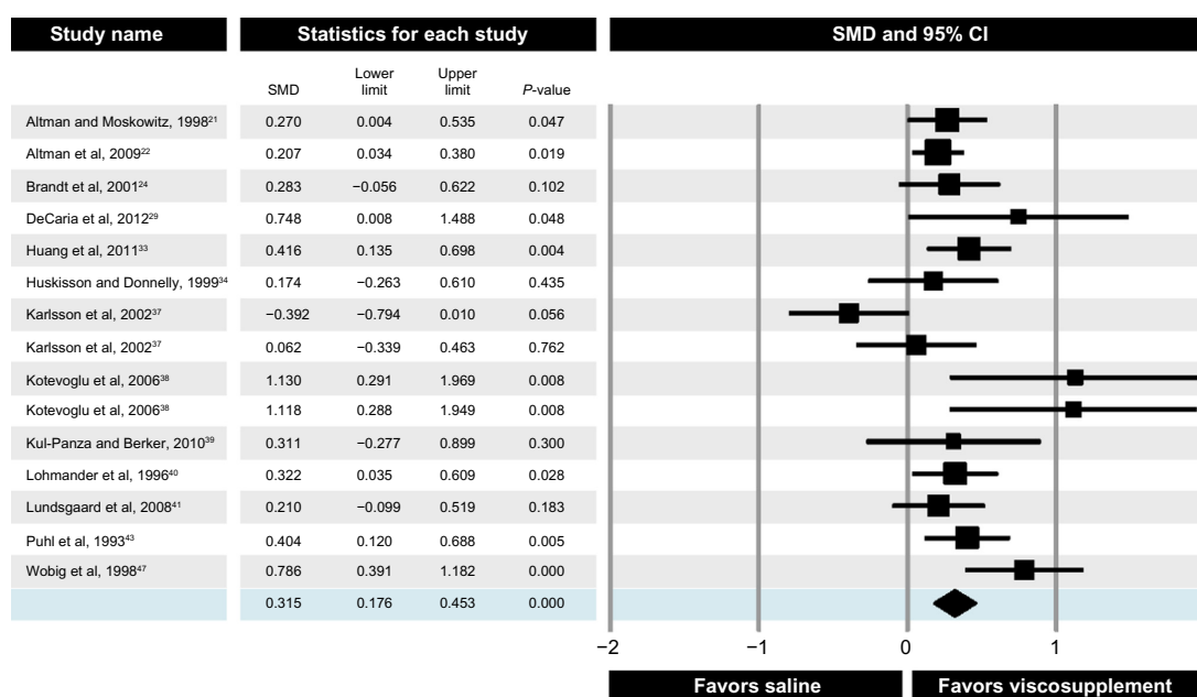
Figure 3 Forest plot of viscosupplementation versus saline controls on knee function at 14 to 26 weeks.
