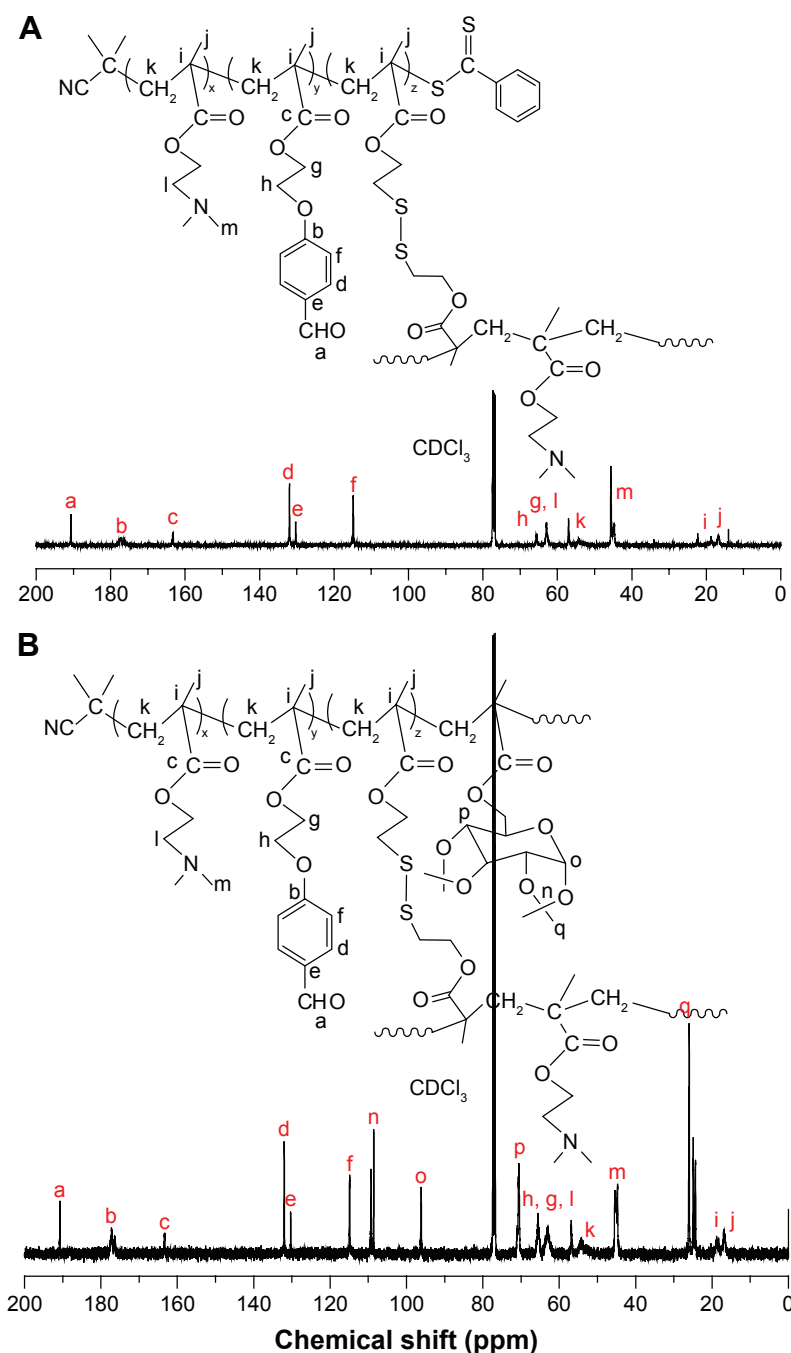
Figure 3 ^{13}\text{C} -NMR spectra of the branched polymer, BP-3 (A), and the branched star polymer, BSP-3 (B).
