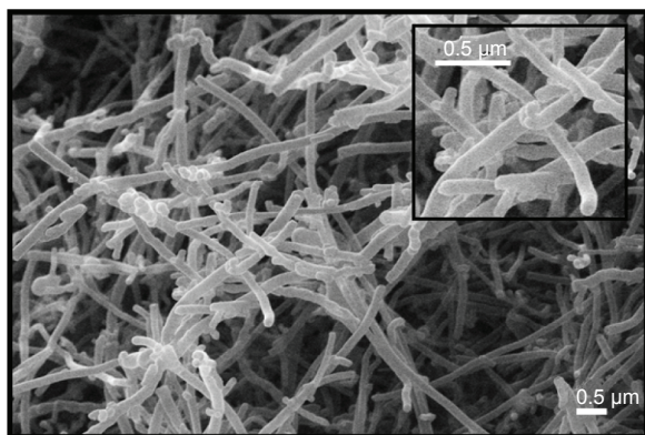
Figure 1 Scanning electron microscopic images of carbon nanofiber (CNF). Notes: The diameter of CNFs is approximately 150–200 nm, and the length of CNFs is approximately 3–15 µm. The scale bars correspond to 0.5 µm.
